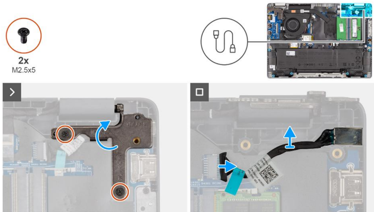
Figure 32. Removing the power-adapter port
