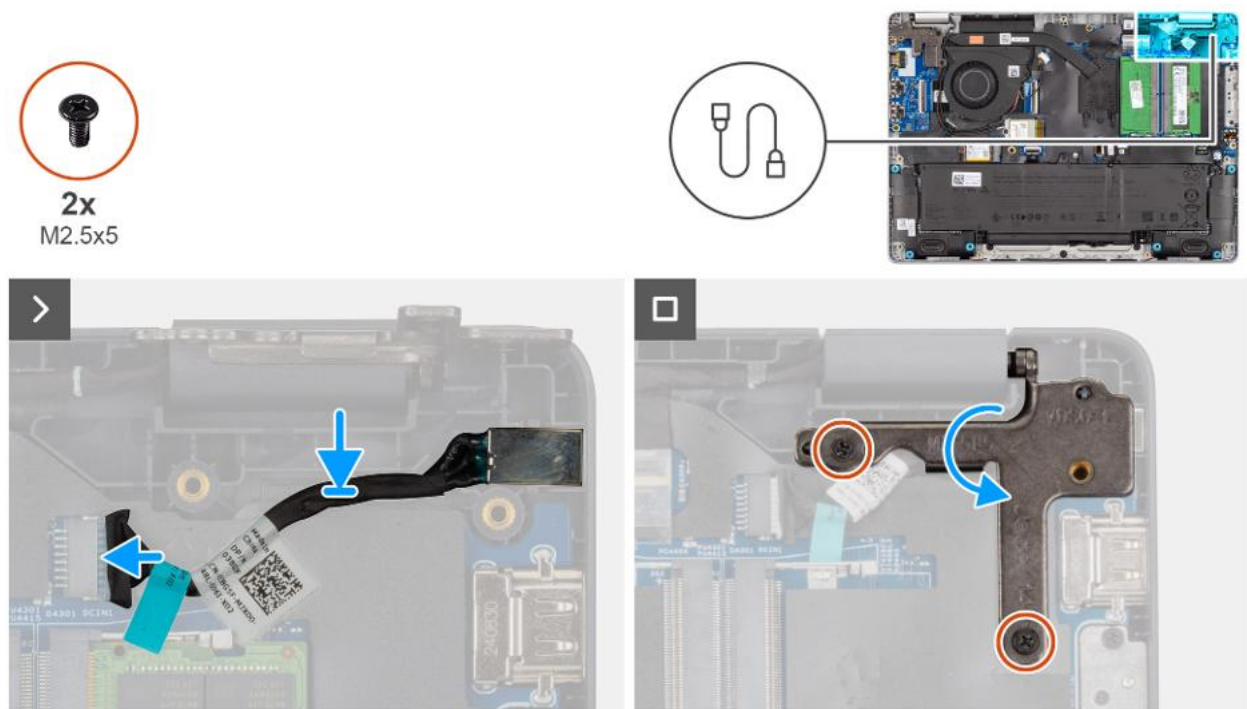
Figure 33. Installing the power-adapter port
