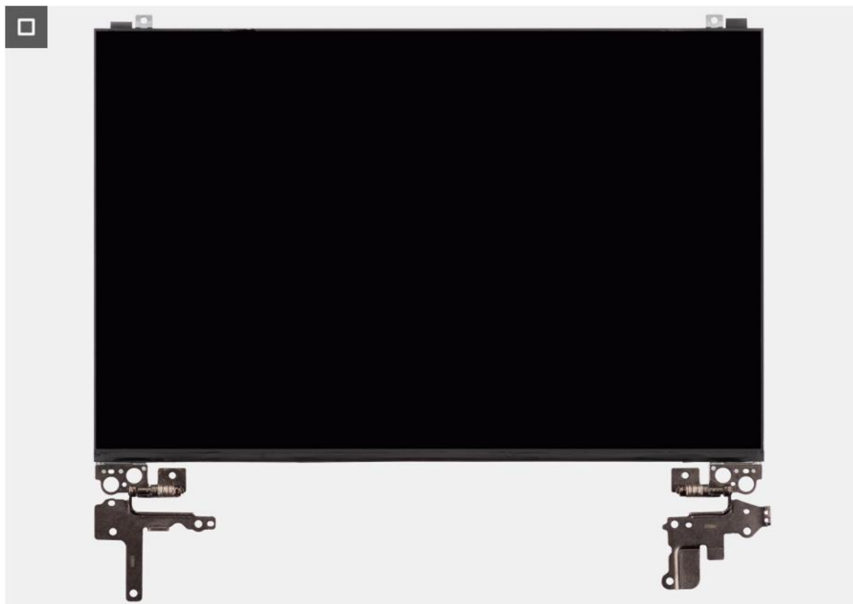
Figure 77. Removing the display-panel assembly
