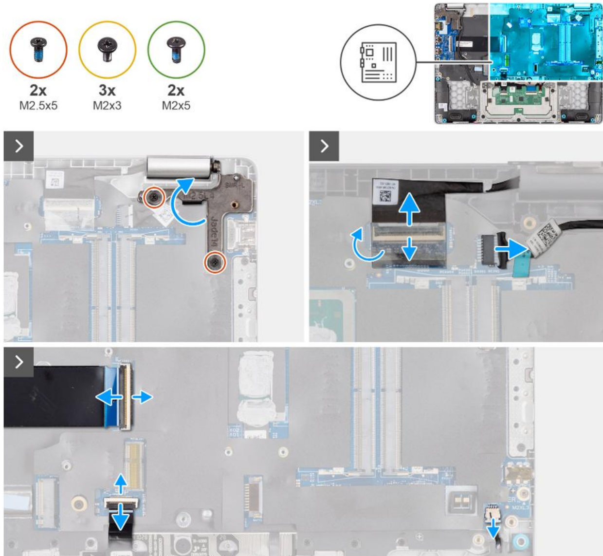
Figure 43. Removing the system board
