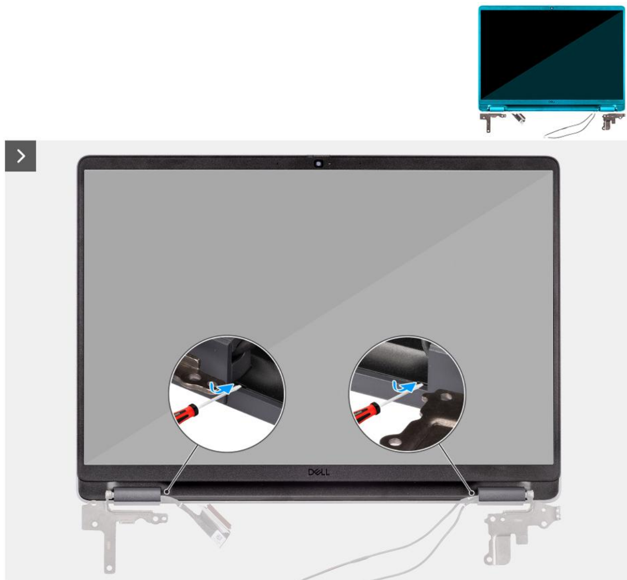
Figure 67. Removing the display bezel
