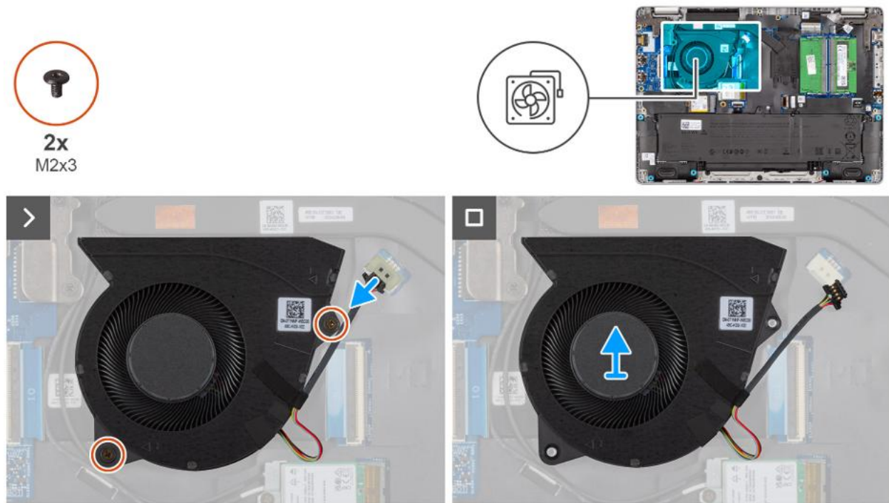
Figure 30. Removing the fan
